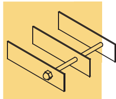
100mm SPACING
