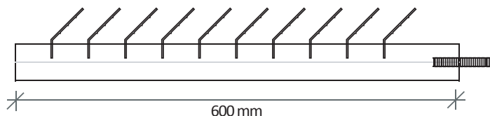
MILLENNIUM SUPER POST 50*50mm ANODIZED OR POWDER COATED
